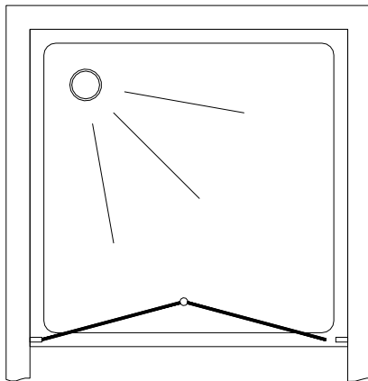
Bi-fold Standard Operation
